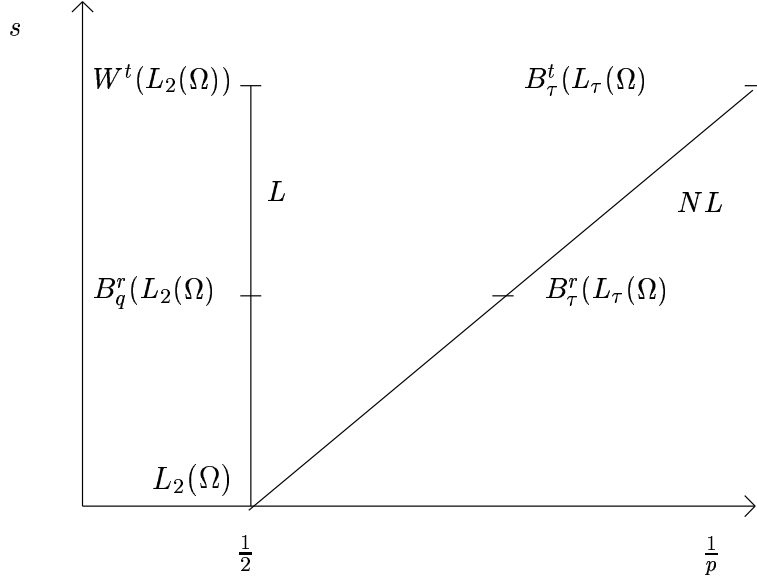
Figure 3.2: Smoothness space diagram
