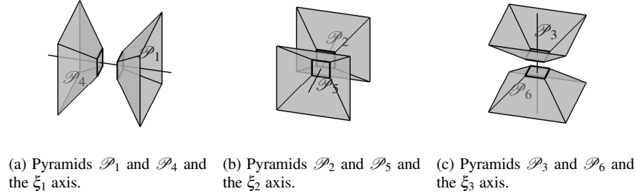
Fig. 6 The partition of the frequency domain: The ‘top’ of the six pyramids.
