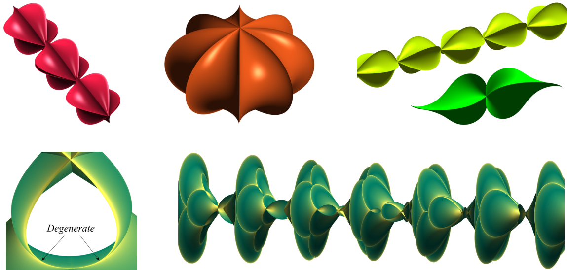
Figure 7: Top: surfaces generated by plane curves with \kappa(s) = \cos^3(s) (left), \kappa(s) = \cos(as) for special values of a (middle two), and \kappa(s) = s . Bottom: Viviani figure-8 space curve.
