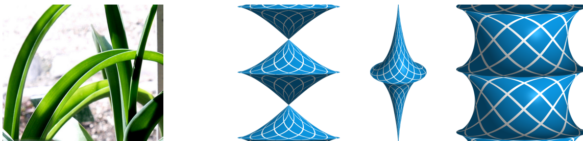
Figure 4: A plant with negatively curved leaves, and the three types of constant negative curvature surfaces of revolution, with asymptotic curves shown. The middle one is the pseudosphere.
